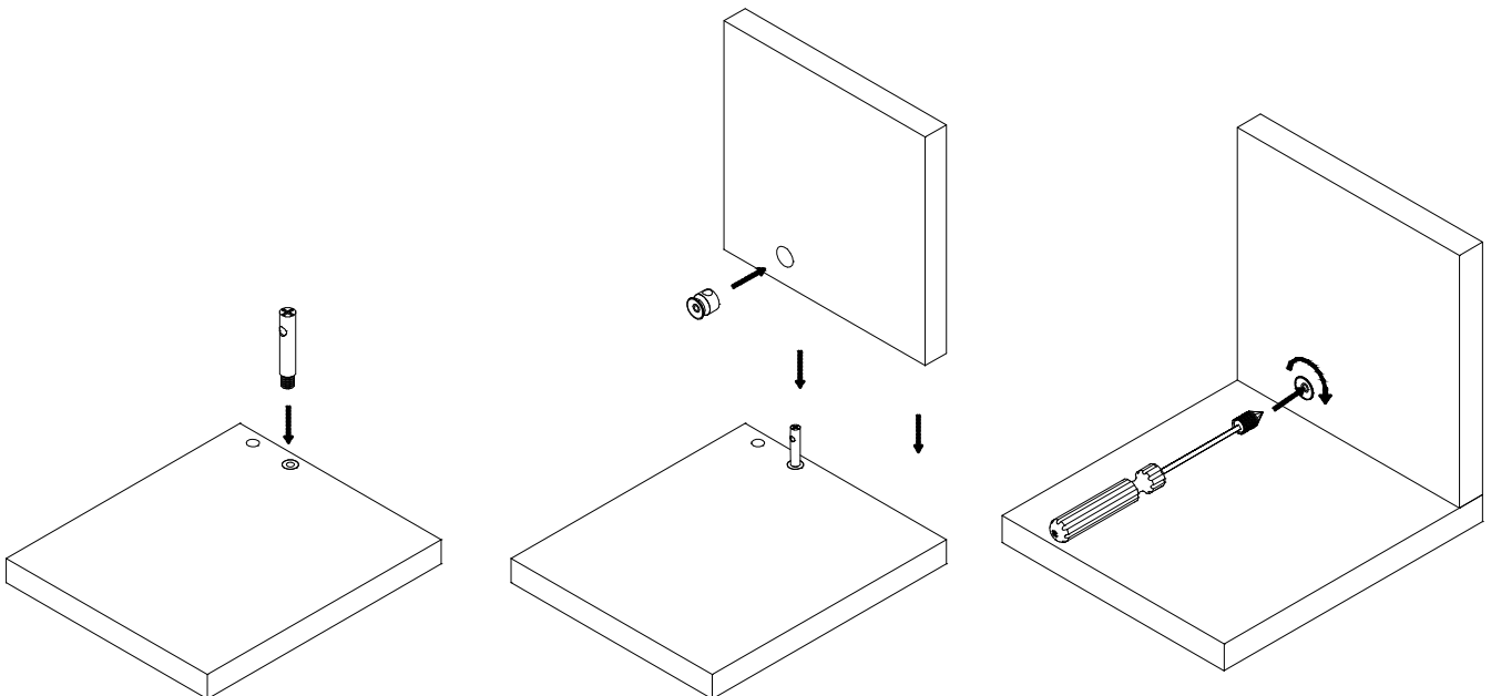
Excenter with 2 holes
